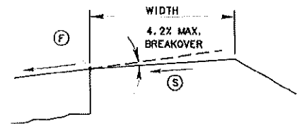
SUPERELEVATED SECTIONS-HIGH SIDE
