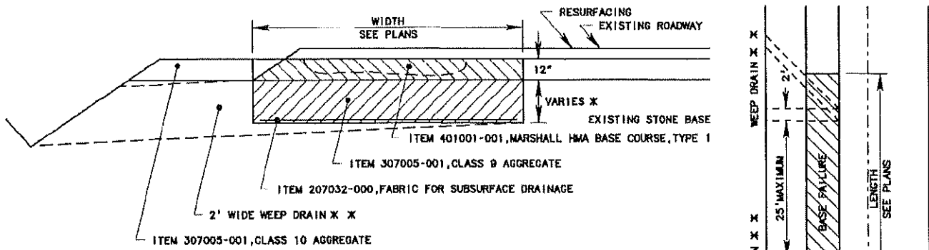
(ELEVATION VIEW)
